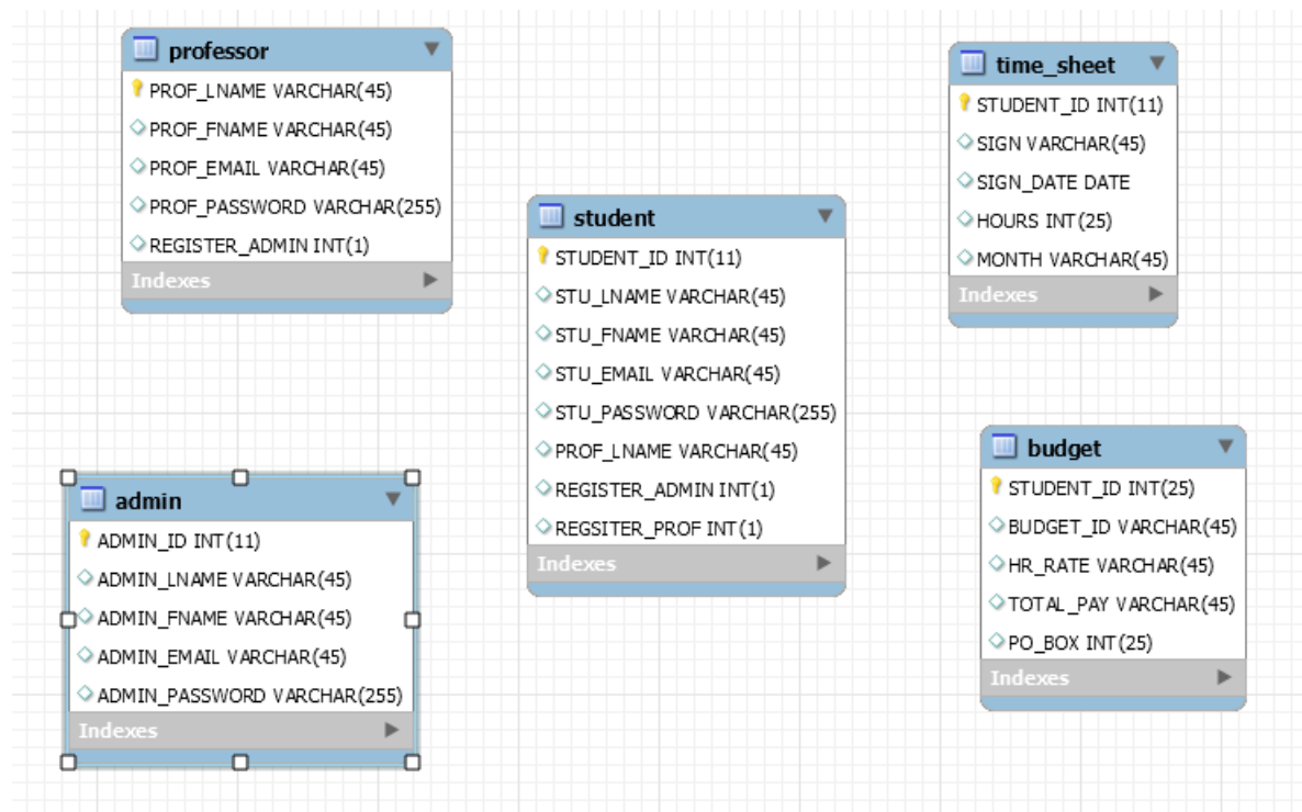
Figure 1 Tables Used to Create the Final ERD
