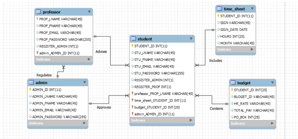
Figure 5 Final ERD Diagram
